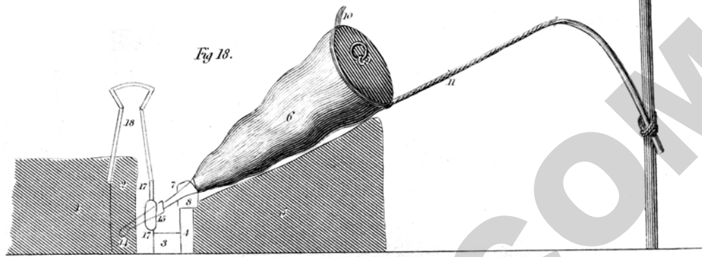
Longitudinal section of the smelting apparatus.
