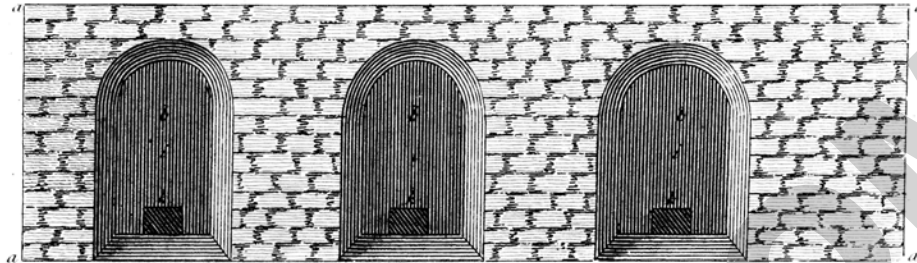
Front view of three glass furnaces.
