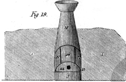
Front view of the smelting furnace.
