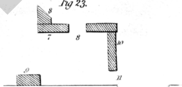
Longitudinal section of the forging furnace.
